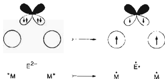
Figure 6. Diagram of the mechanism of anion-mediated superexchange. The central anion ( E^{2-} ) is shown with two perpendicular valence p-orbitals, and each metal atom is represented by a single s-orbital for simplicity. The normal anionic configuration is represented at the left. In this configuration each p-orbital is doubly-occupied. The associated reverse-charge-transfer configuration is shown at the right. In this configuration each E-centered p-orbital is singly-occupied. Since the two p-orbitals are orthogonal, the low energy intra-atomic coupling on E is high-spin. This gives the ferromagnetic coupling of the two metal centers.
