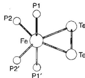
Figure 4. Structure of and labeling for \text{FeTe}_2(\text{depe})_2 , 5. Selected distances and angles are given in Table 5.
