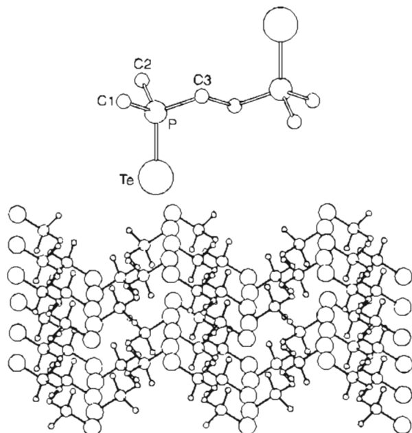
Figure 3. (a) Top: Structure of and labeling for \text{dmpe}\cdot 2\text{Te} . Selected distances and angles are given in Table 4. (b) Bottom: Crystal packing diagram for \text{dmpe}\cdot 2\text{Te} .
